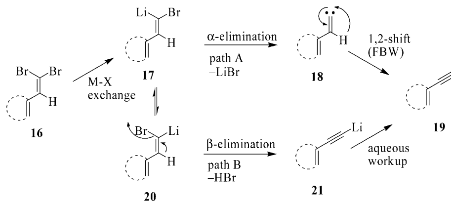
Scheme 4. Proposed mechanistic pathways for the conversion of tetrabromides 12 to enediynes 13 with 16 as the model substrate.
