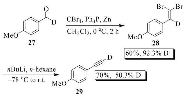
Scheme 6. Mechanistic evaluation of the base-mediated transformation of alkylidene dibromide 28 into the acetylene 29 by a deuterium-labeling experiment.
