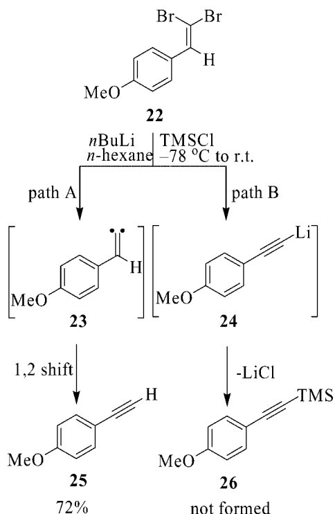
Scheme 5. Treatment of dibromide 22 with n\text{BuLi} and quenching the reaction mixture with \text{TMSCl} .
